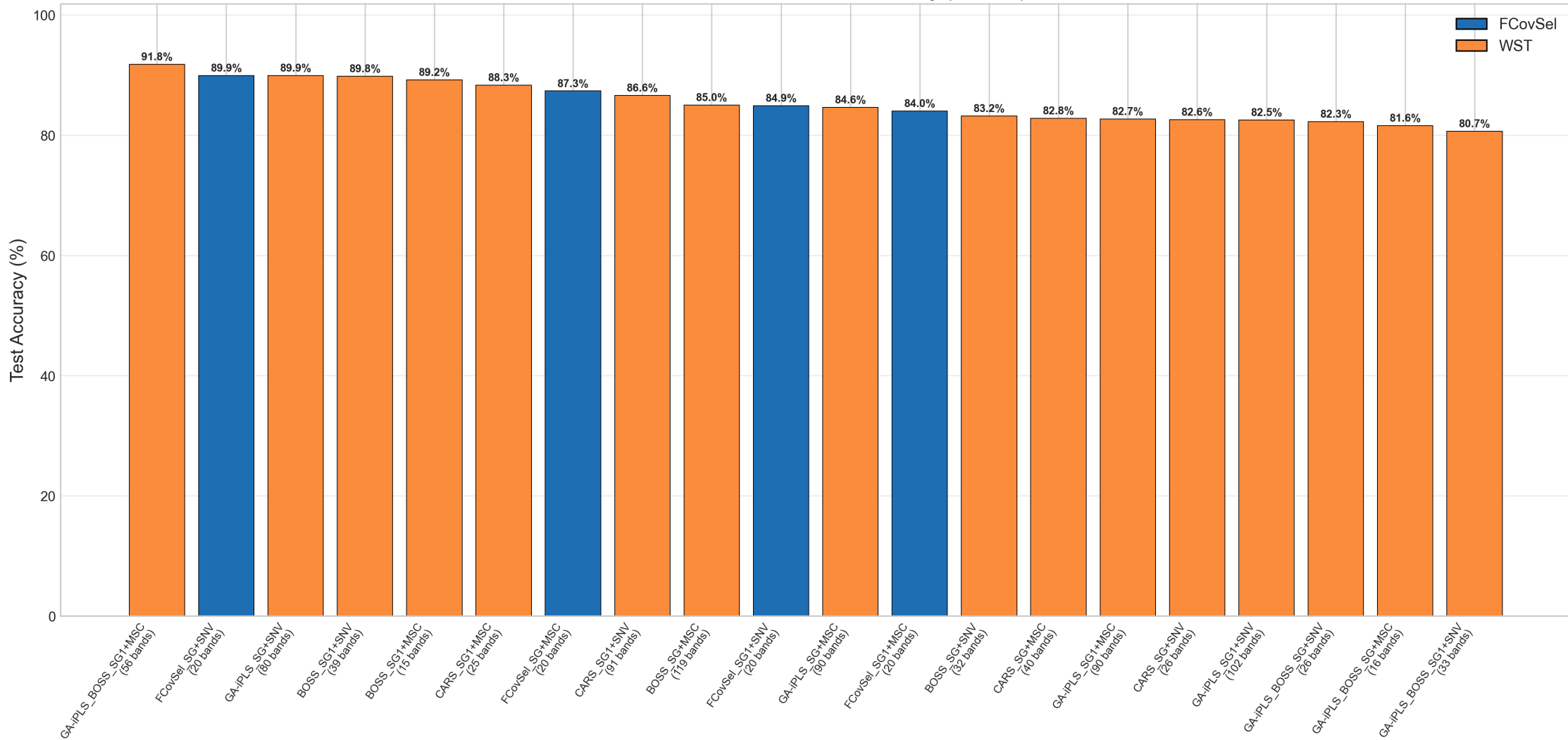
All Methods - 3D-CNN Test Accuracy (Salinas)
